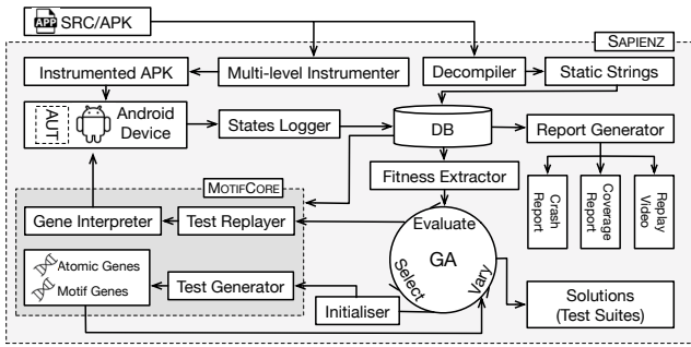
Figure 1: Sapienz workflow.
