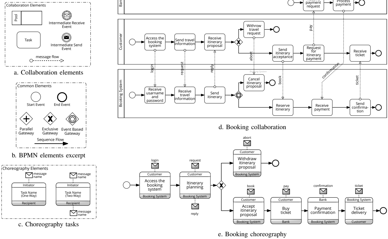
Figure 1. BPMN 2.0 Elements and Booking Example.
